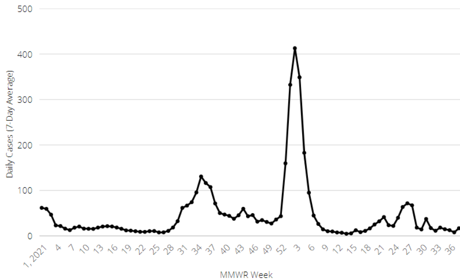
Graph 1: 7-Day Average per Week
